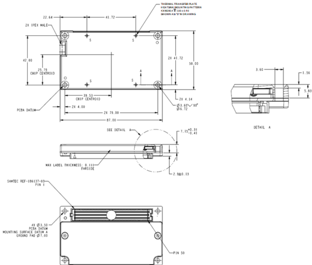
Figure 7 Jetson TX2 Module Package Outline with Dimensions
